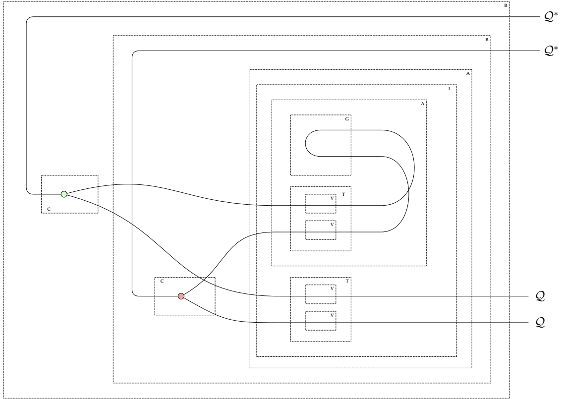
Figure C.1: The CNOT-gate.
