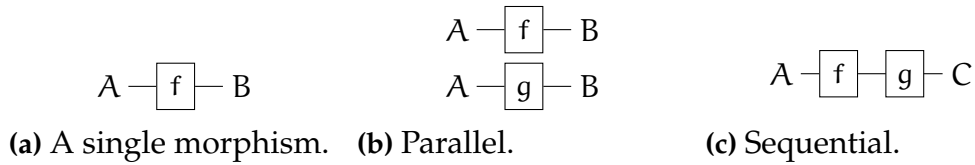
Figure 1.9: Representation of a single morphism, parallel and sequential composition of morphisms in a string diagram.
