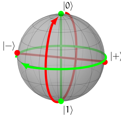
Figure 1.10: The Bloch-sphere with axes of rotation.
