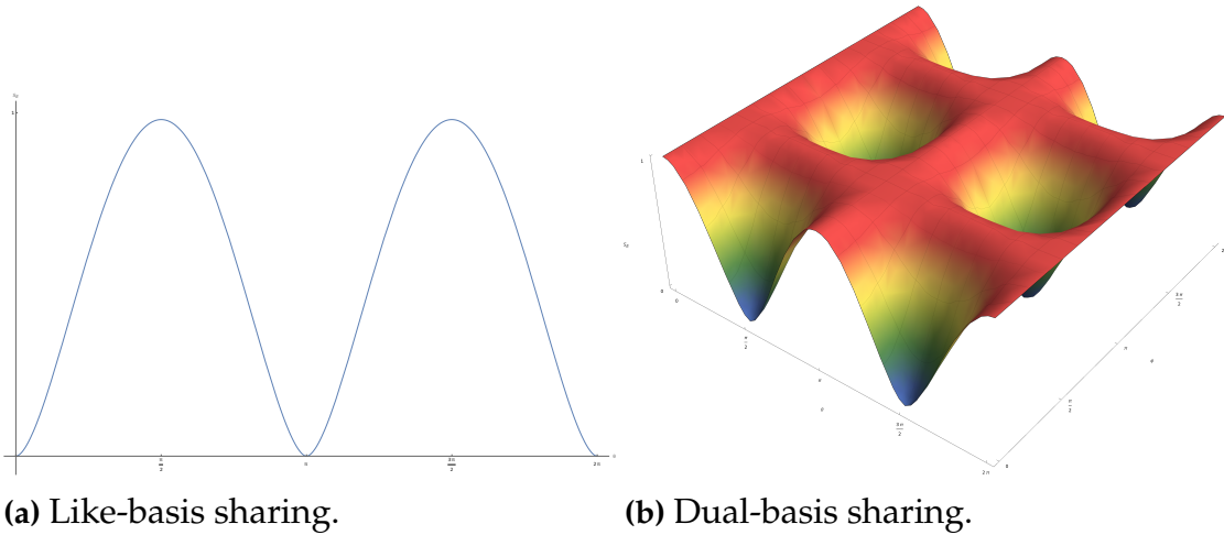
Figure 3.6: Sharing analysis.
