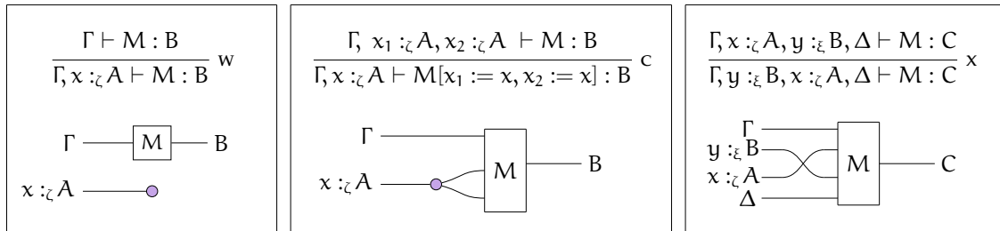
Figure 2.8: Interpretation of structural rules.
