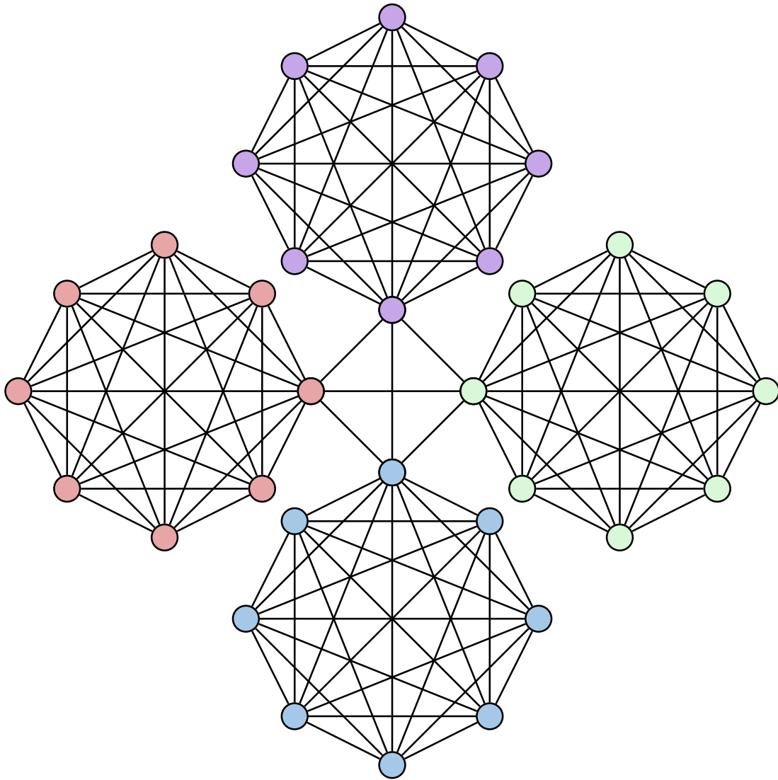
Figure 3.5: Conjectured basis crystal for \mathfrak{X}_4 .
